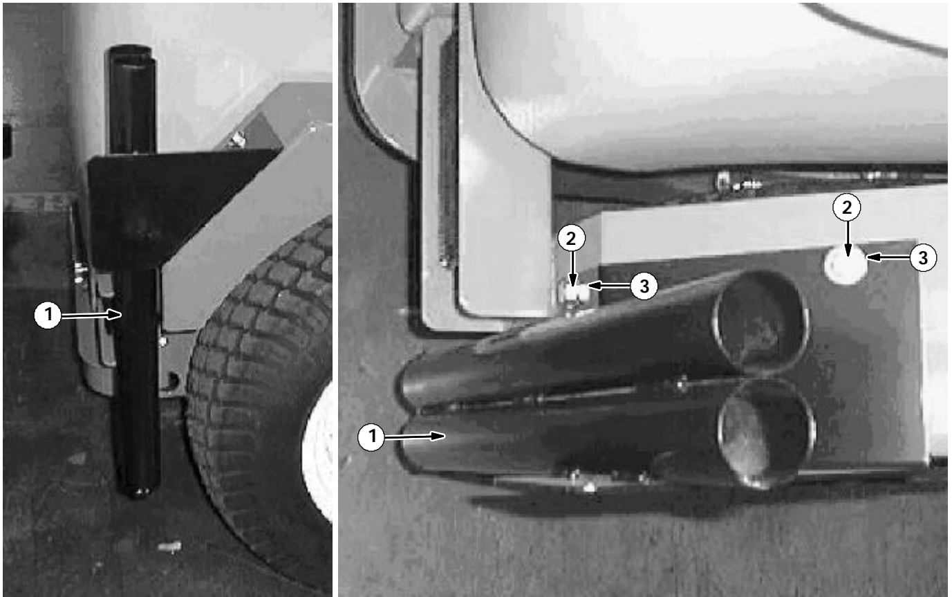
FIG. 2 - BROOM HOLDER KIT INSTALLATION
